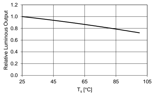
SOLDER POINT TEMPERATURE VS RELATIVE LUMINOUS OUTPUT ( I_F = 60\text{ mA} )
