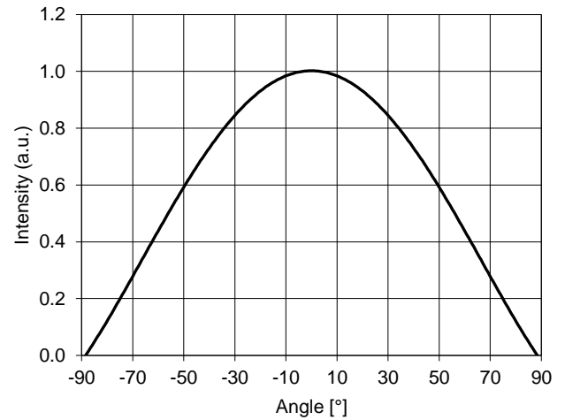
TYPICAL SPATIAL DISTRIBUTION ( T_A = 25^\circ\text{C} , I_F = 60 mA)
