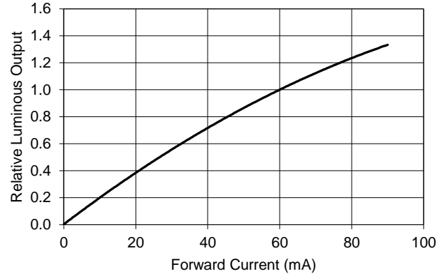
FORWARD CURRENT VS RELATIVE LUMINOUS OUTPUT ( T_A = 25^\circ )
