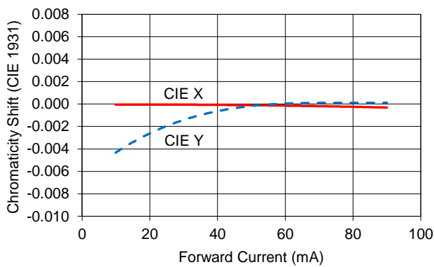
FORWARD CURRENT VS CHROMATICITY SHIFT (3200K, T_A = 25^\circ\text{C} )
