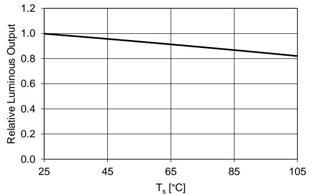
SOLDER POINT TEMPERATURE VS RELATIVE LUMINOUS OUTPUT ( I_F = 300\text{ mA} )
