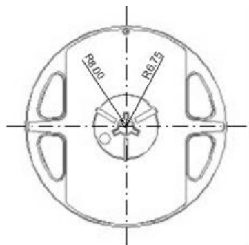
Reel dimensions side (unit: mm)
