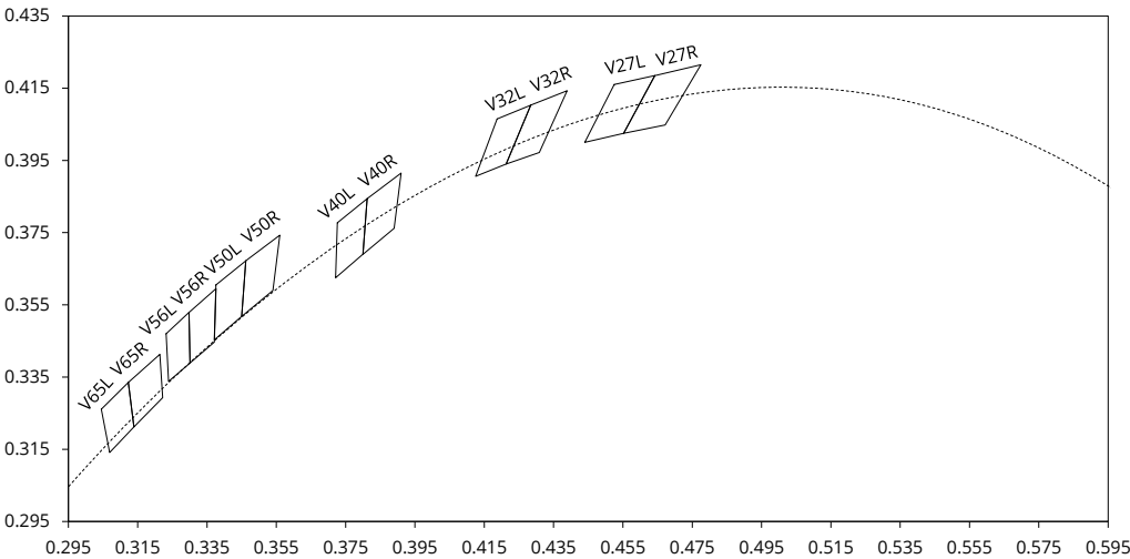
CIE 1931 diagram
