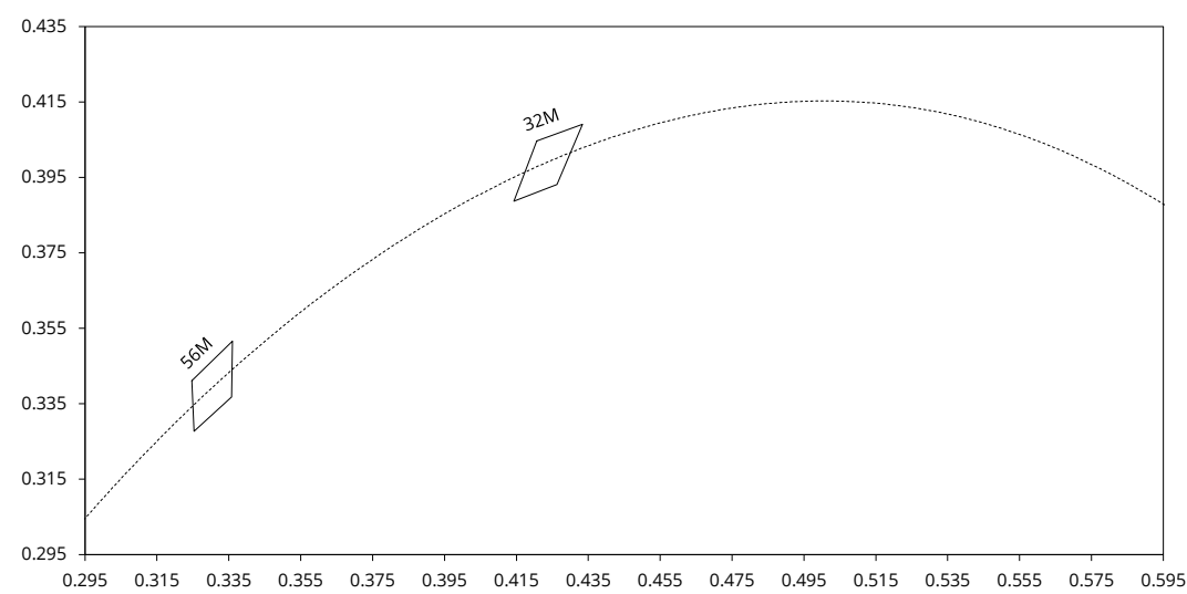
CIE 1931 diagram
