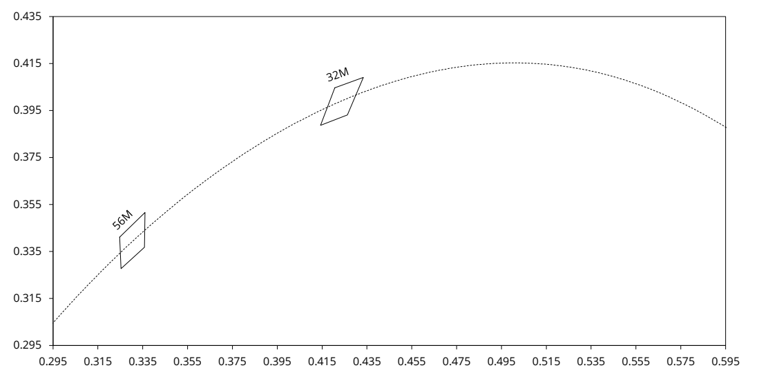
CIE 1931 diagram
