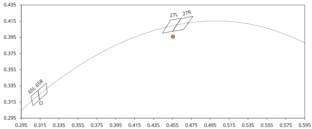
CIE 1931 diagram
